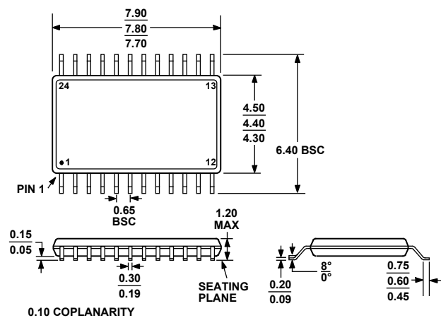
COMPLIANT TO JEDEC STANDARDS MO-153-AD Figure 45. 24-Lead Thin Shrink Small Outline Package [TSSOP] (RU-24) Dimensions shown in millimeters
