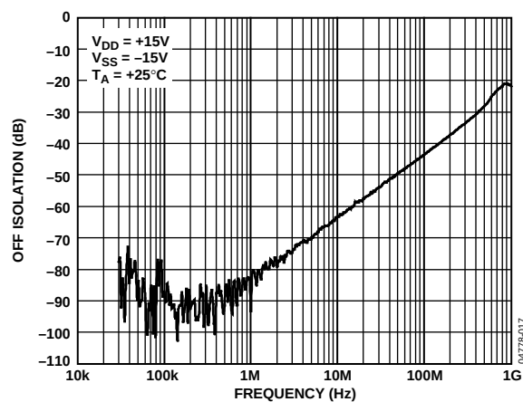
Figure 14. Off Isolation vs. Frequency
