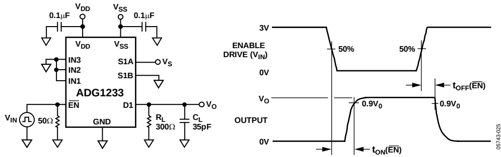
Figure 28. Enable Delay, t_{ON}(\overline{EN}) , t_{OFF}(\overline{EN})
