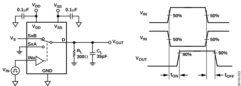
Figure 26. Switching Timing
