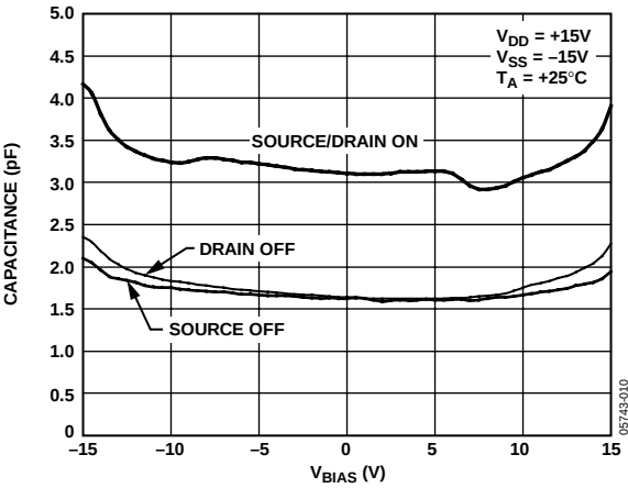
Figure 20. Capacitance vs. Source Voltage for Dual Supply
