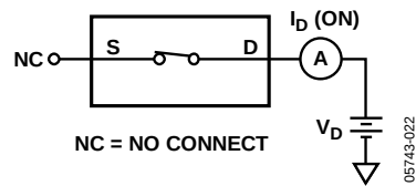
Figure 25. On Leakage
