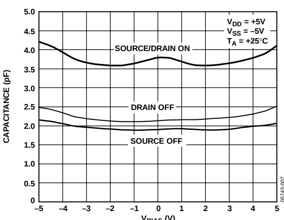
Figure 22. Capacitance vs. Source Voltage for Dual Supply
