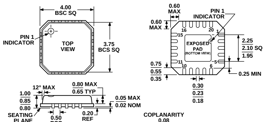
Figure 37. 20-Lead Lead Frame Chip Scale Package [LFCSP_VQ] 4 mm × 4 mm Body, Very Thin Quad (CP-20-1) Dimensions shown in millimeters
