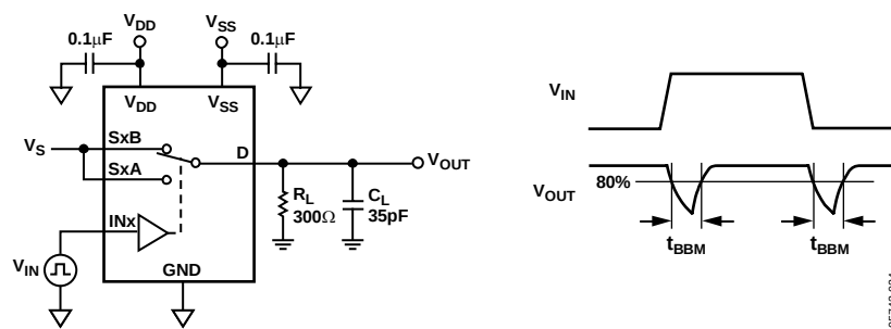
Figure 27. Break-Before-Make Delay
