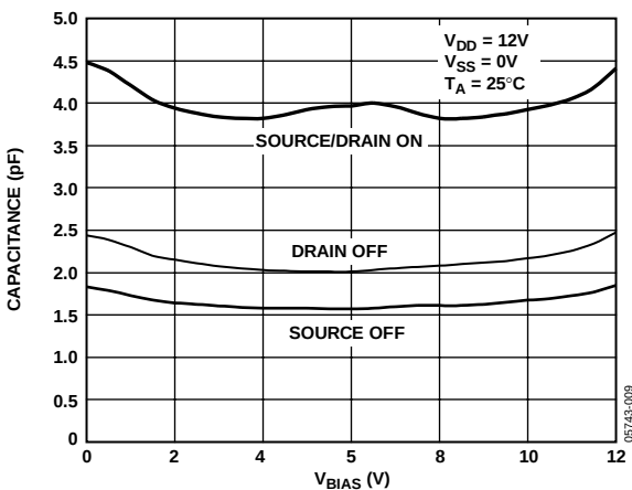
Figure 21. Capacitance vs. Source Voltage for Single Supply
