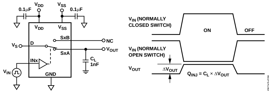
Figure 29. Charge Injection
