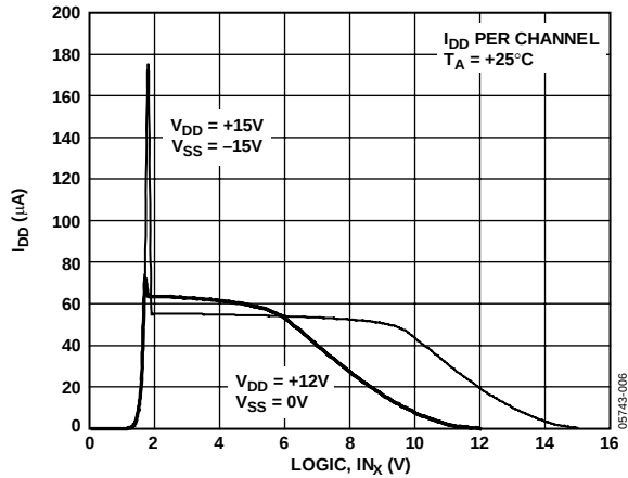
Figure 13. I_{\text{DD}} vs. Logic Level
