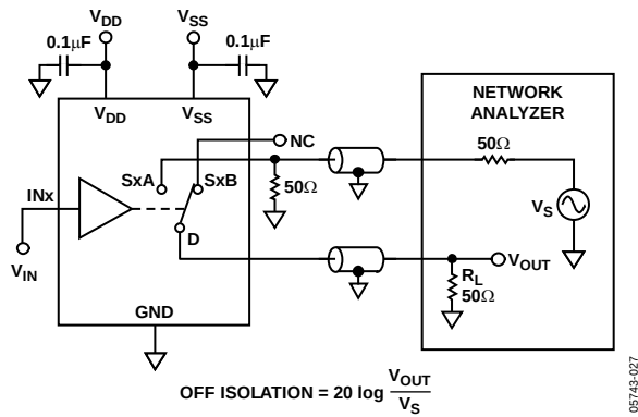
Figure 30. Off Isolation
