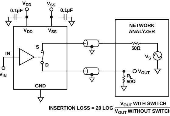
Figure 26. Bandwidth
