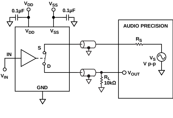
Figure 27. THD + N
