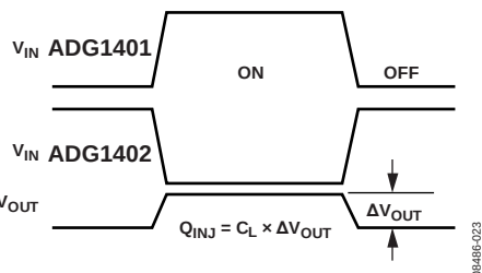
Figure 24. Charge Injection
