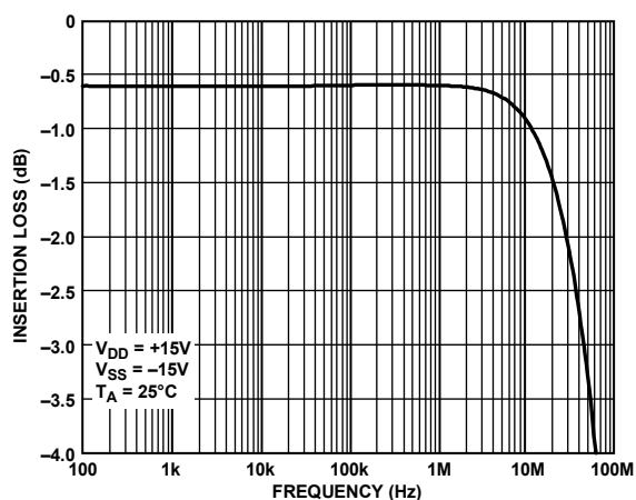
Figure 23. ADG1406 On Response vs. Frequency
