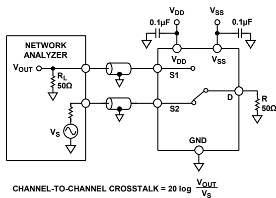
Figure 36. Channel-to-Channel Crosstalk
