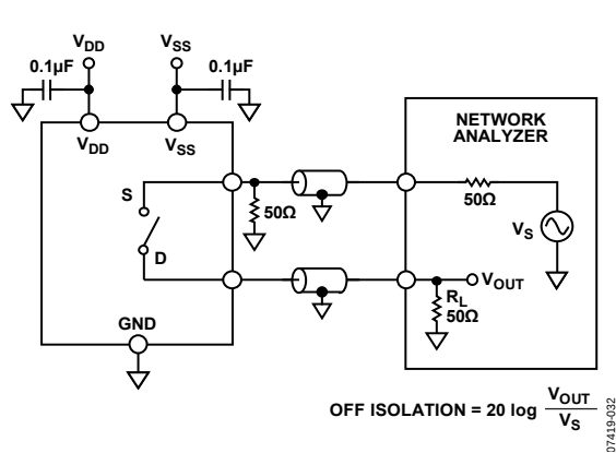
Figure 34. Off Isolation
