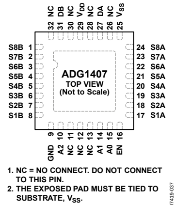
Figure 6. ADG1407 LFCSP Pin Configuration
