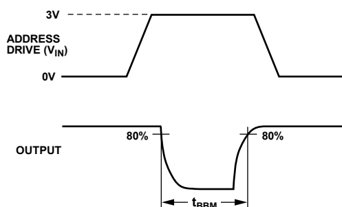
Figure 31. Break-Before-Make Delay, t_{\text{BBM}}
