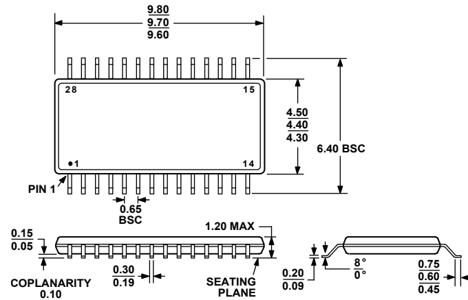
Figure 38. 28-Lead Thin Shrink Small Outline Package [TSSOP] (RU-28)
