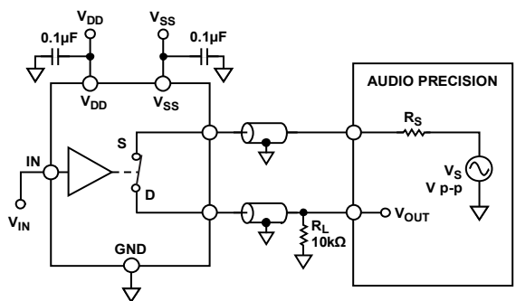
Figure 37. THD + Noise
