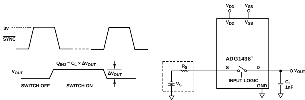
Figure 32. Charge Injection
