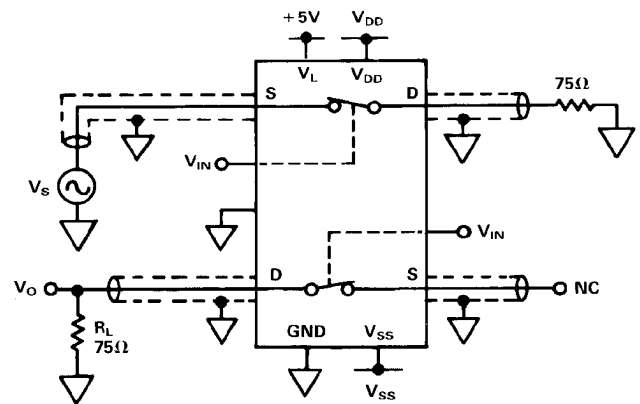
Test Circuit 7. Channel-to-Channel Crosstalk
