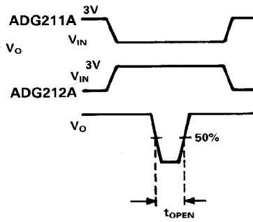
Test Circuit 3
