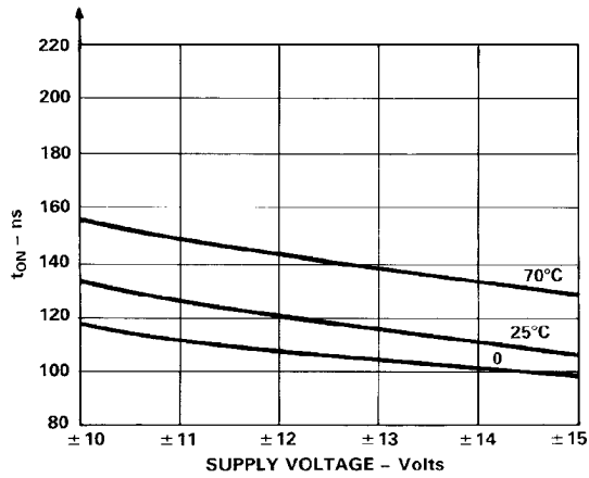
Figure 7. t_{ON} vs. Supply Voltage, (Dual Supply)
