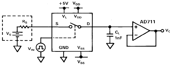
Test Circuit 8. Charge Injection
