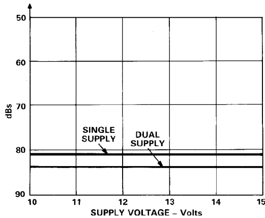
Figure 11. Off Isolation and Channel-to-Channel Crosstalk vs. Supply Voltage
