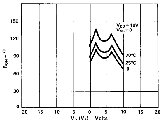
Figure 4. R_{ON} as a Function of V_D (V_S) : Single +10V Supply
