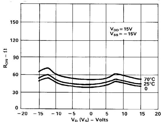
Figure 1. R_{ON} as a Function of V_D (V_S) : Dual \pm 15 Supplies
