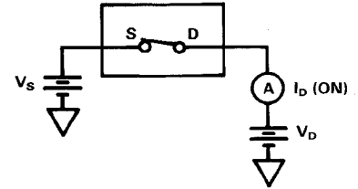
Test Circuit 3
