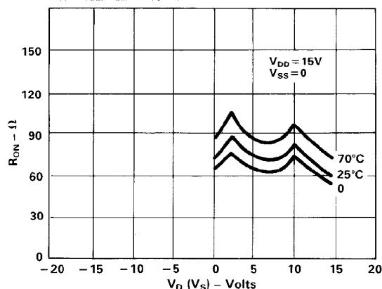
Figure 2. R_{ON} as a Function of V_D (V_S) : Single +15V Supply
