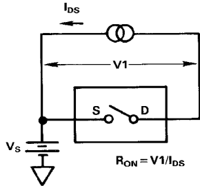
Test Circuit 1
