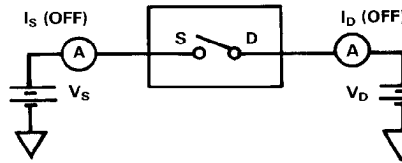
Test Circuit 2
