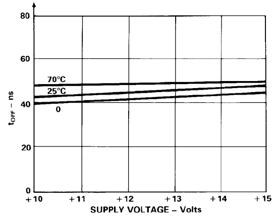
Figure 10. t_{OFF} vs. Supply Voltage, (Single Supply)
