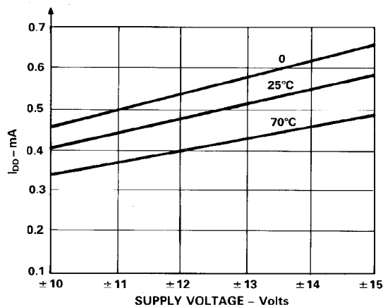
Figure 14. I_{DD} vs. Supply Voltage, (Dual Supply)
