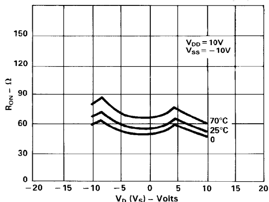
Figure 3. R_{ON} as a Function of V_D (V_S) : Dual \pm 10 V Supplies
