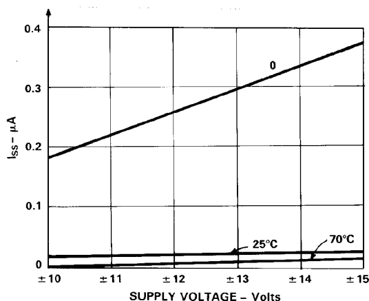
Figure 15. I_{SS} vs. Supply Voltage, (Dual Supply)
