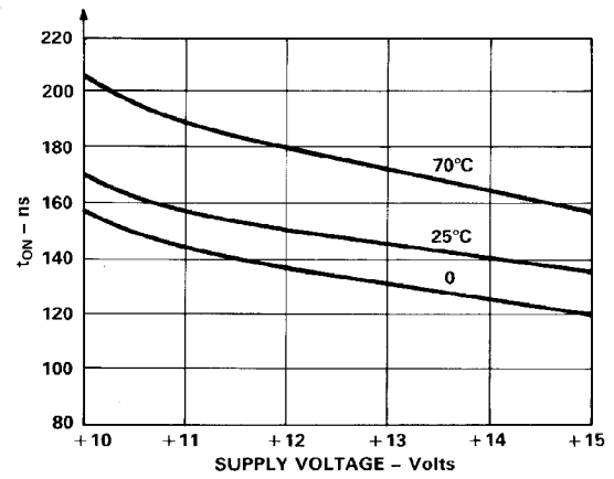
Figure 8. t_{ON} vs. Supply Voltage, (Single Supply)
