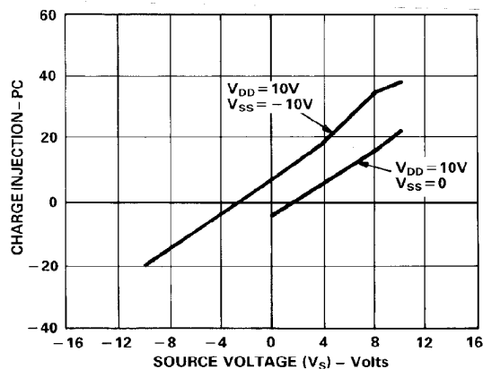
Figure 13. Charge Injection vs. Source Voltage for Dual and Single 10V Supplies
