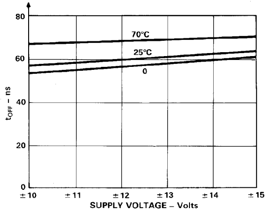
Figure 9. t_{OFF} vs. Supply Voltage, (Dual Supply)
