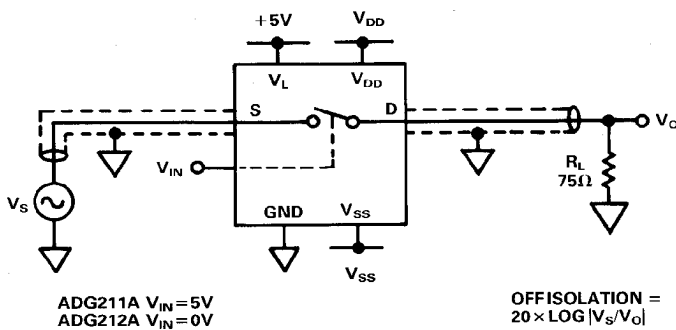
Test Circuit 6. Off Isolation
