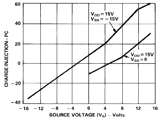
Figure 12. Charge Injection vs. Source Voltage ( V_S ) for Dual and Single 15V Supplies
