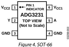
Figure 4. SOT-66
