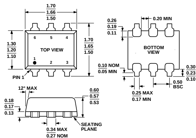
Figure 21. 6-Lead Small Outline Transistor Package [SOT-66] (RY-6-1) Dimensions shown in millimeters
