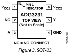
Figure 3. SOT-23
