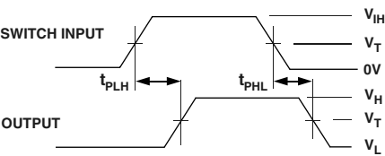
Figure 2. Propagation Delay
