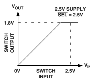
Figure 8. 2.5 V to 1.8 V Voltage Translation, \overline{SEL} = V_{CC}
