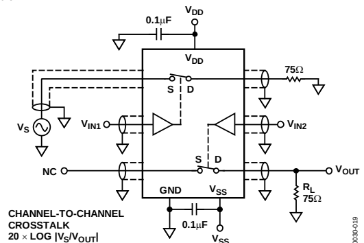
Figure 19. Channel-to-Channel Crosstalk
