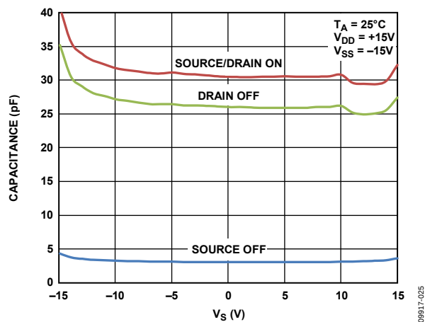
Figure 25. ADG5209 Capacitance vs. Source Voltage, \pm 15\text{ V} Dual Supply
