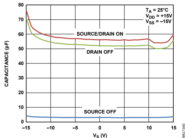
Figure 26. ADG5208 Capacitance vs. Source Voltage, \pm 15\text{ V} Dual Supply
