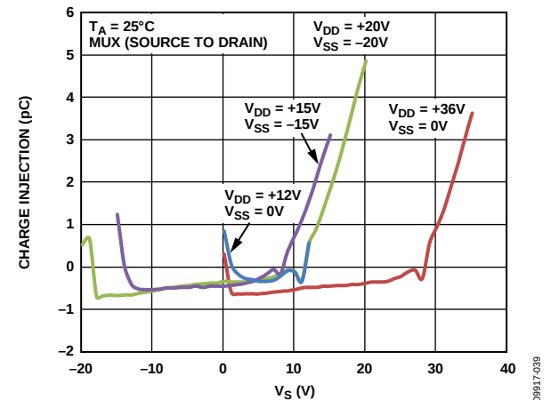
Figure 23. Charge Injection vs. Source Voltage, Source to Drain
