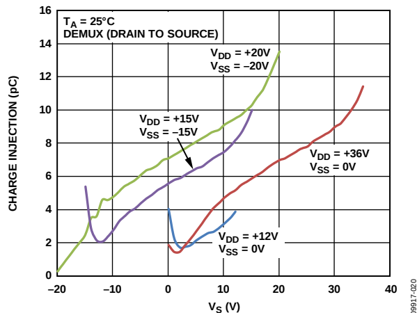
Figure 20. Charge Injection vs. Source Voltage, Drain to Source
