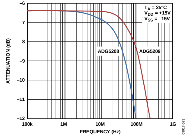
Figure 22. Bandwidth
