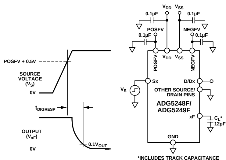
Figure 43. Interrupt Flag Response Time, t_{\text{DIGRESP}}
