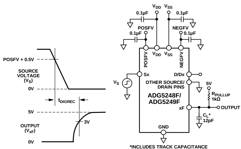
Figure 45. Interrupt Flag Recovery Time, t_{DIGREC} , with a 1 kΩ Pull-Up Resistor
