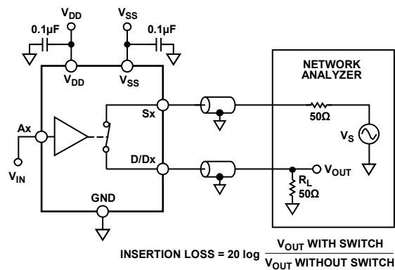
Figure 40. Bandwidth
