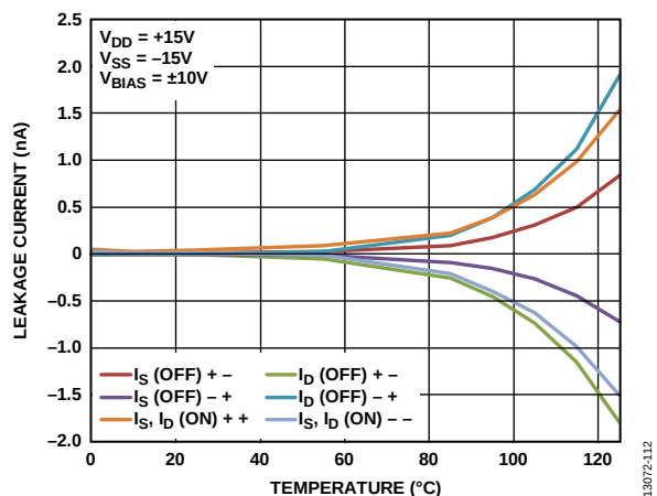
Figure 12. Leakage Current vs. Temperature, \pm 15 V Dual Supply
