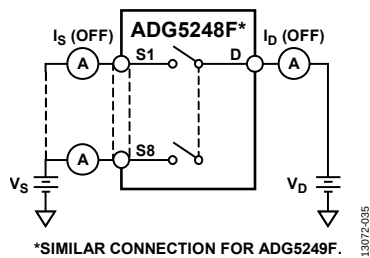
Figure 34. Off Leakage
