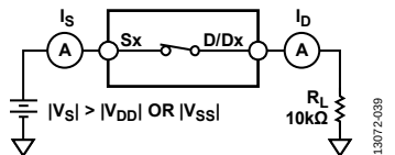
Figure 33. Switch Overvoltage Leakage
