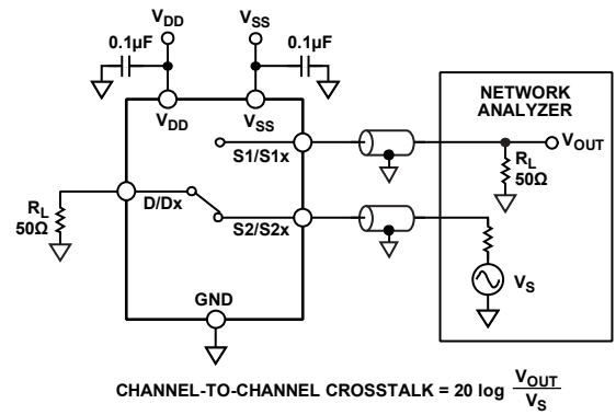
Figure 38. Channel-to-Channel Crosstalk
