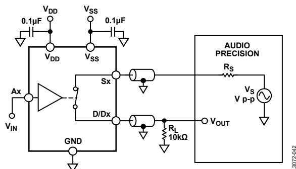
Figure 37. THD + N
