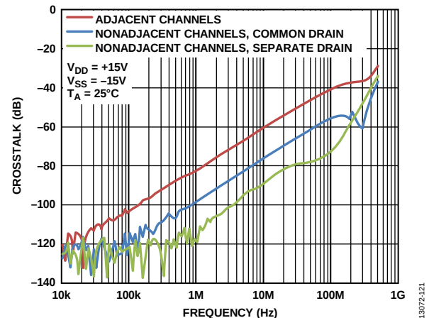
Figure 21. Crosstalk vs. Frequency, \pm 15 V Dual Supply
