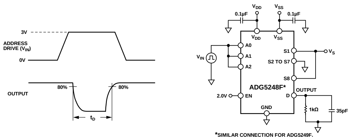
Figure 46. Break-Before-Make Time Delay, t_b
