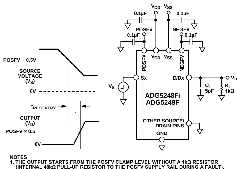
Figure 42. Overvoltage Recovery Time, t_{\text{RECOVERY}}
