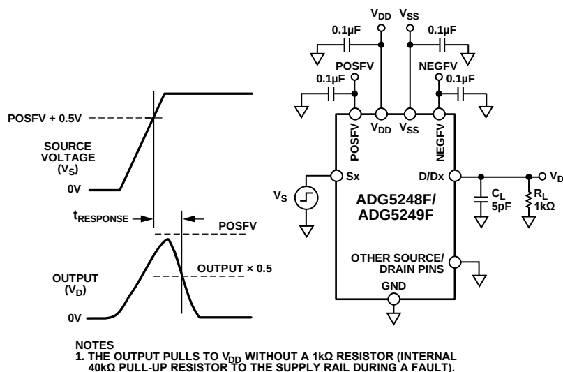
Figure 41. Overvoltage Response Time, t_{\text{RESPONSE}}
