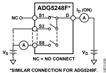
Figure 35. On Leakage
