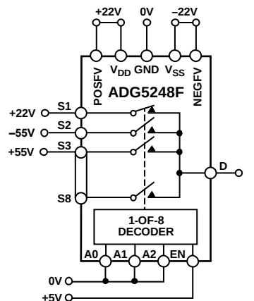
Figure 52. ADG5248F in an Overvoltage Condition
