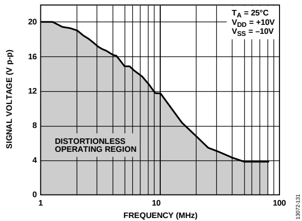
Figure 31. Large Signal Voltage Tracking vs. Frequency
