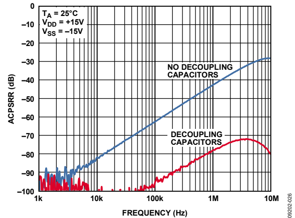
Figure 19. ACPSR vs. Frequency, \pm 15 V Dual Supply
