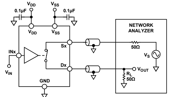
Figure 29. Bandwidth
