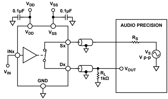
Figure 28. THD + Noise
