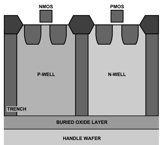
Figure 33. Trench Isolation
