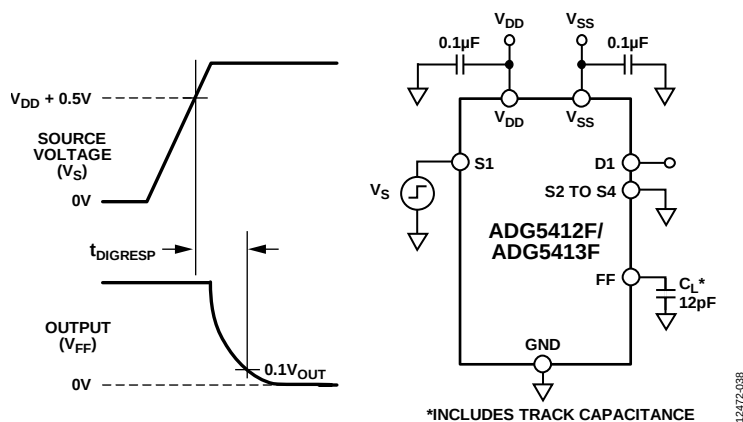
Figure 42. Interrupt Flag Response Time, t_{\text{DIGRESP}}
