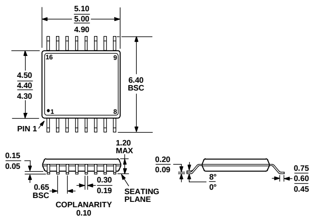
Figure 51. 16-Lead Thin Shrink Small Outline Package [TSSOP] (RU-16)
