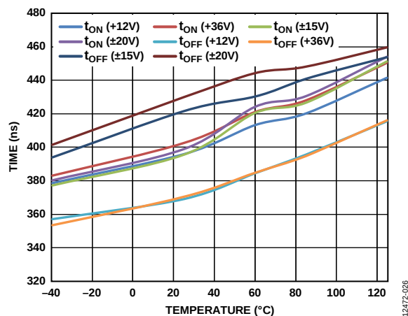
Figure 26. t_{ON} , t_{OFF} Times vs. Temperature
