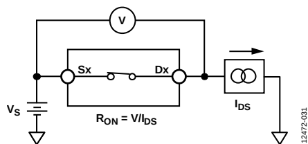
Figure 31. On Resistance
