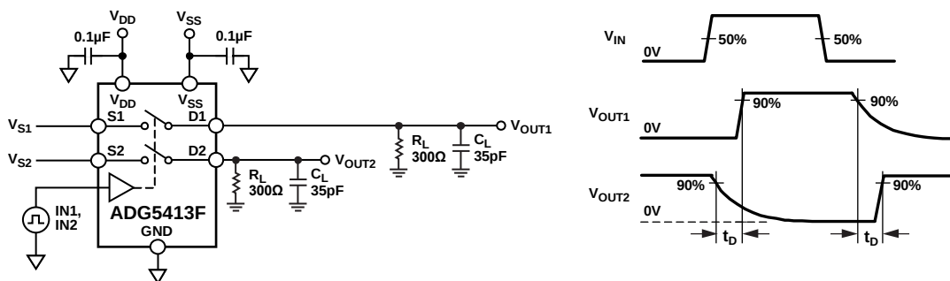
Figure 45. Break-Before-Make Time Delay, t_D
