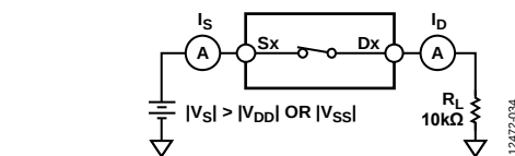
Figure 36. Switch Overvoltage Leakage
