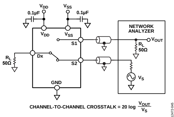
Figure 35. Channel-to-Channel Crosstalk
