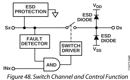
Figure 48. Switch Channel and Control Function
