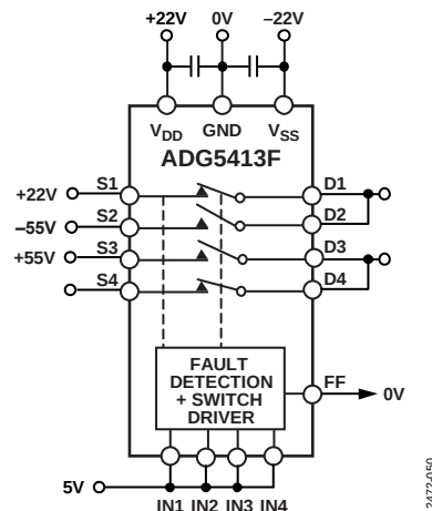
Figure 50. ADG5413F in Multiplexer Configuration under Overvoltage Conditions
