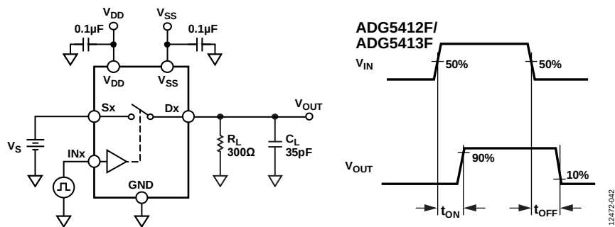
Figure 46. Switching Times, t_{ON} and t_{OFF}
