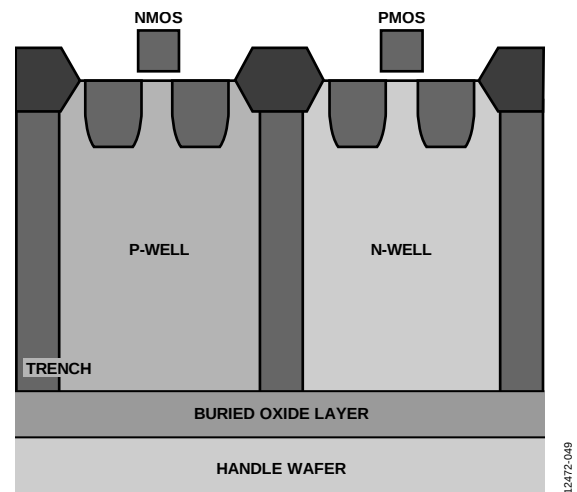
Figure 49. Trench Isolation
