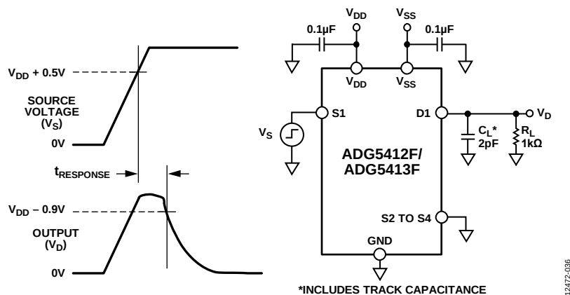
Figure 40. Overvoltage Response Time, t_{\text{RESPONSE}}
