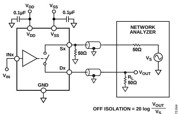
Figure 34. Off Isolation
