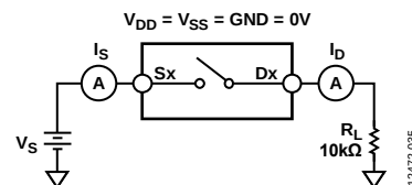
Figure 37. Switch Unpowered Leakage
