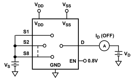
Figure 22. I_D (OFF)
