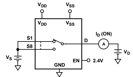
Figure 23. I_D (ON)
