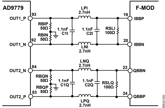
Figure 30. DAC Modulator Interface with 3 MHz Third-Order, Low-Pass Filter
