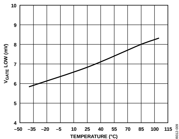
Figure 9. V_{GATE\ Low} vs. Temperature ( I_{GATE} = 100\text{ }\mu\text{A} )
