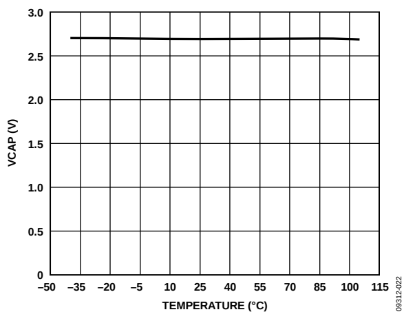
Figure 22. VCAP vs. Temperature ( I_{VCAP} = 100 \mu A )
