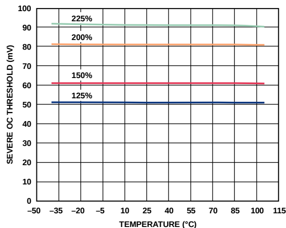
Figure 36. Severe OC Threshold vs. Temperature, ADM1075-2 , I_{SET} = 1.65\text{ V}
