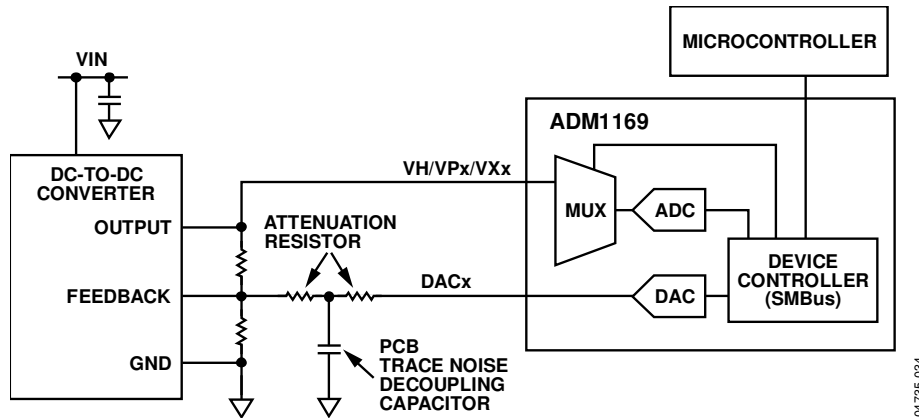
Figure 33. Closed-Loop Margining System Using the ADM1169
