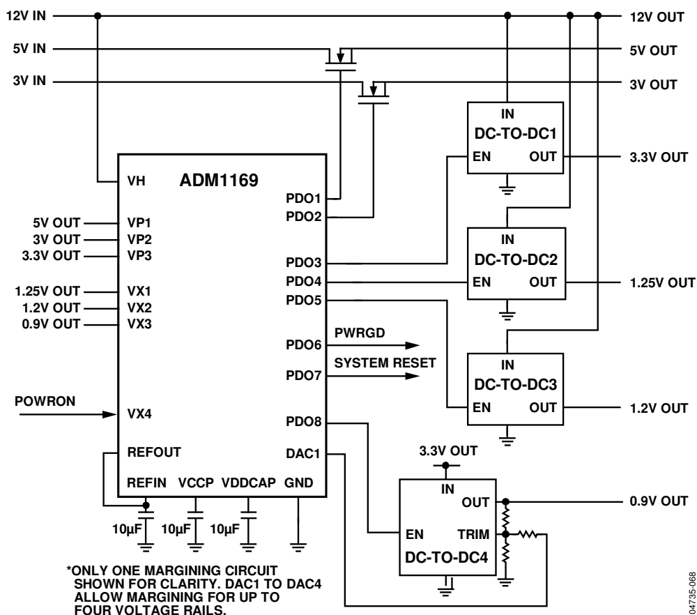
Figure 34. Applications Diagram
