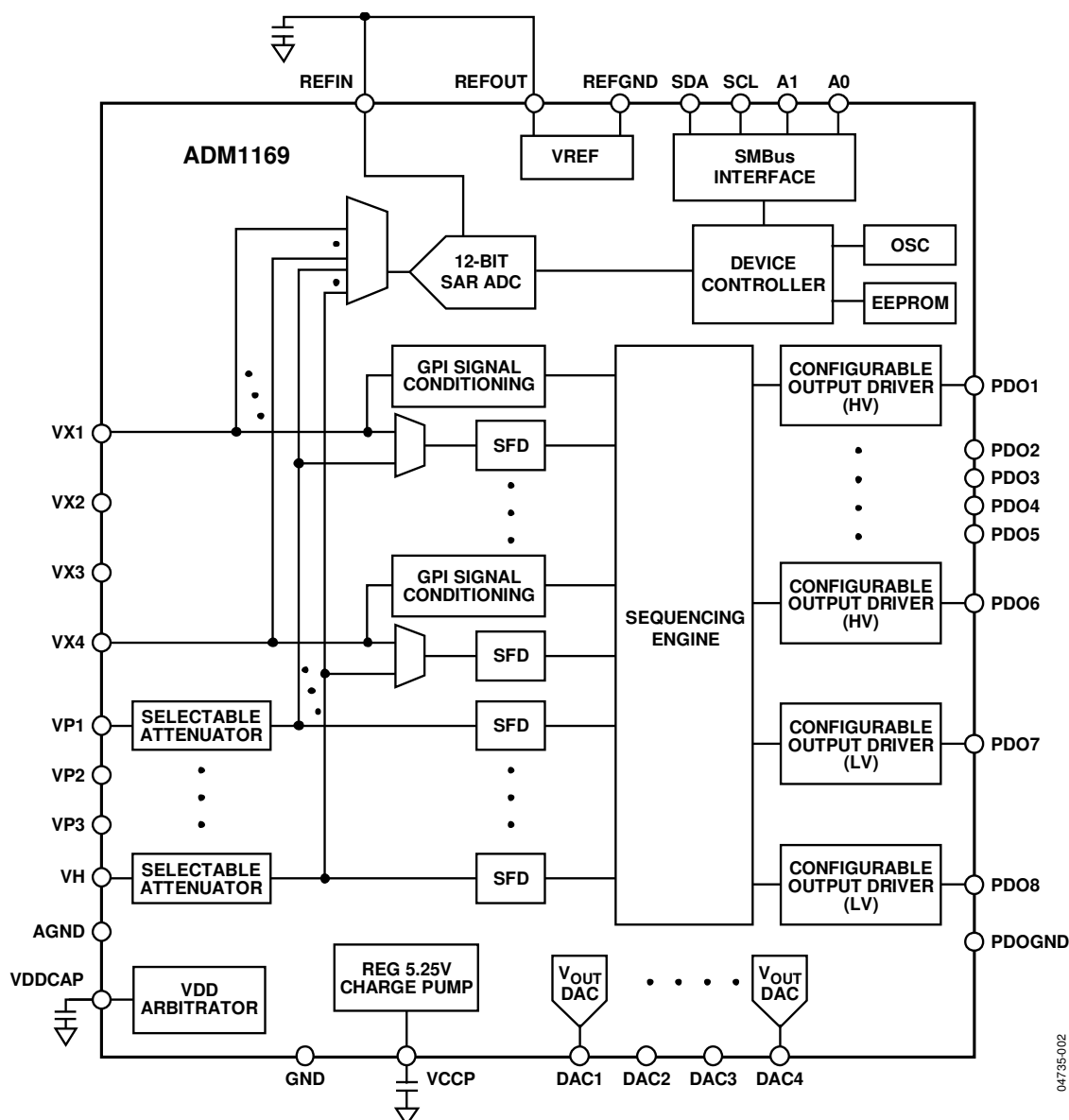
Figure 2. Detailed Block Diagram
