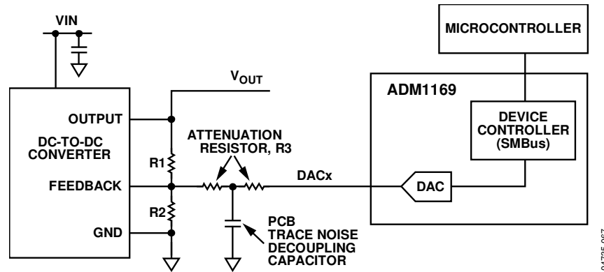
Figure 32. Open-Loop Margining System Using the ADM1169
