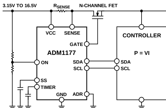
Figure 2. Applications Diagram
