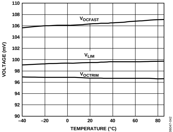
Figure 23. V OCTRIM , V LIM , V OF vs. Temperature
