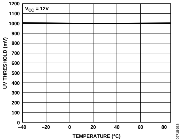
Figure 35. UV Threshold ( UV_{TH} ) vs. Temperature
