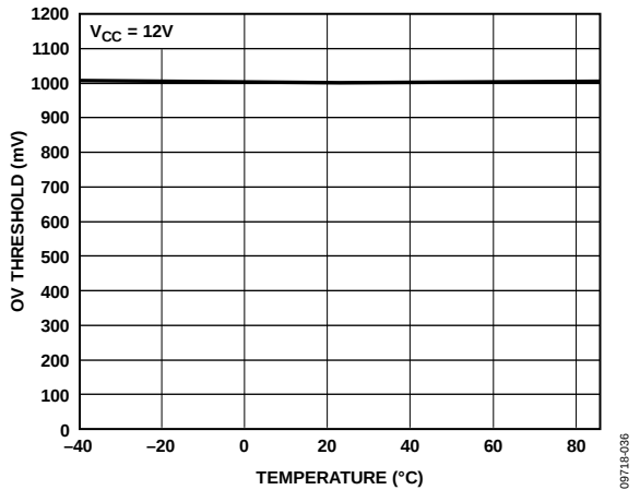
Figure 36. OV Threshold ( OV_{TH} ) vs. Temperature
