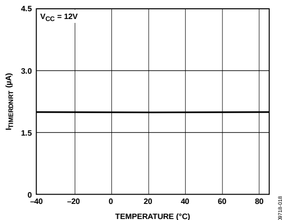
Figure 18. Timer Pull-Down Current, Retry ( I_{\text{TIMERDNRT}} ) vs. Temperature
