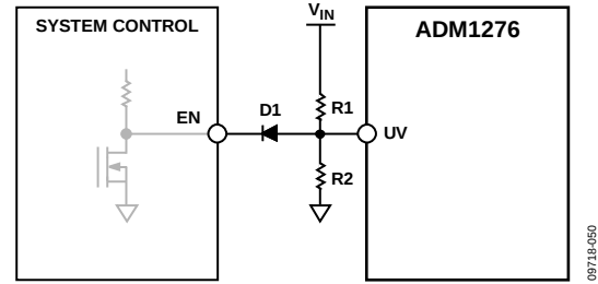
Figure 50. Using the UV Pin as an Enable
