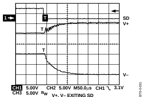
Figure 26. Charge Pump V+ and V- Exiting Shutdown
