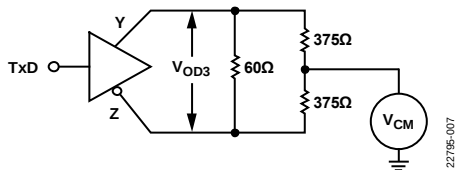
Figure 31. Driver Voltage Measurement over Common-Mode Range, |V_{OD3}|
