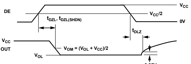
Figure 11. Driver Enable and Disable Times ( t_{DZL} , t_{DLZ} , t_{DZL(SHDN)} )
