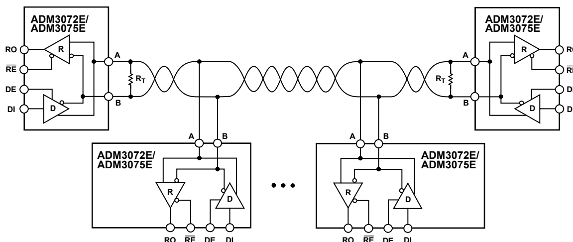
Figure 34. ADM3072E/ADM3075E Typical Half-Duplex RS-485 Network
