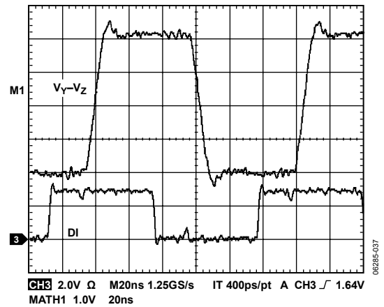
Figure 31. ADM3076E Driver Propagation Delay (16 Mbps)
