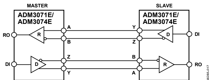
Figure 35. ADM3071E/ADM3074E Full-Duplex Point-to-Point Applications
