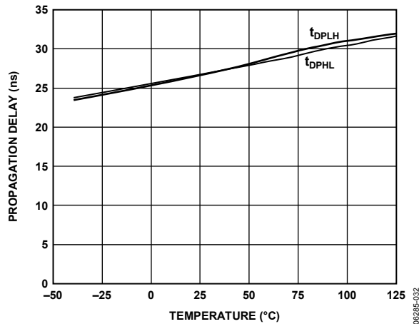
Figure 27. ADM3076E Driver Propagation Delay vs. Temperature (16 Mbps)
