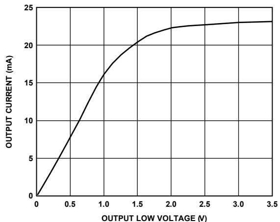
Figure 17. Output Current vs. Receiver Output Low Voltage
