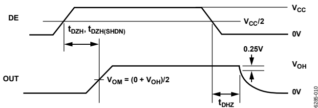
Figure 10. Driver Enable and Disable Times ( t_{DZH} , t_{DZH(SHDN)} , t_{DHZ} )
