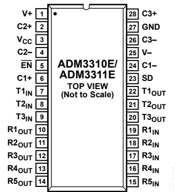
Figure 7. SSOP/TSSOP Pin Configuration
