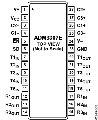
Figure 5. SSOP/TSSOP Pin Configuration
