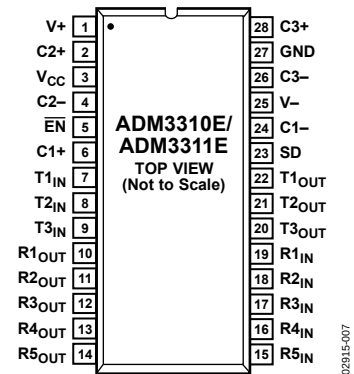
Figure 7. SSOP/TSSOP Pin Configuration
