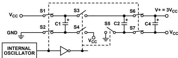
Figure 24. Charge Pump Voltage Tripler
