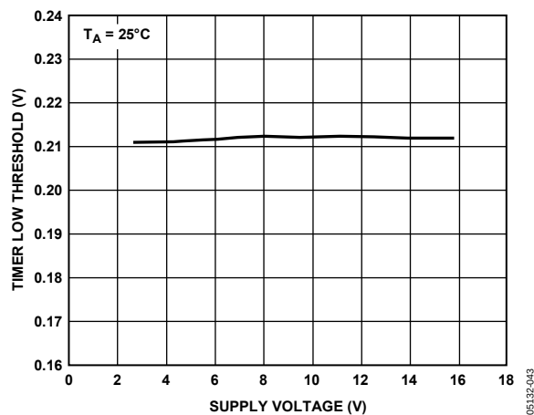
Figure 22. TIMER Low Threshold vs. Supply Voltage
