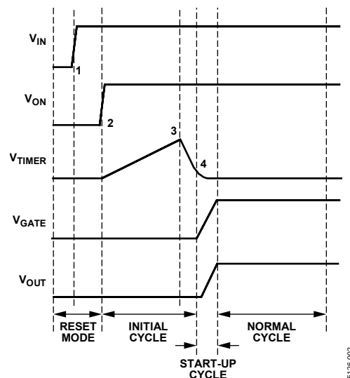
Figure 30. Power-Up Timing
