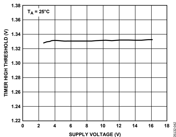
Figure 20. TIMER High Threshold vs. Supply Voltage
