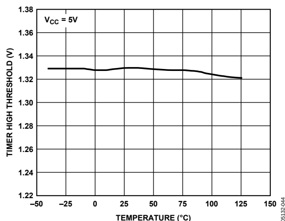
Figure 21. TIMER High Threshold vs. Temperature
