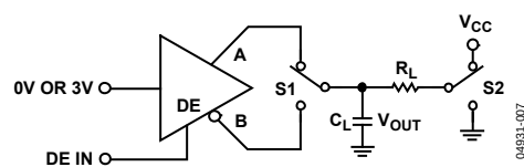
Figure 21. Driver Enable/Disable
