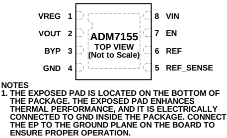
Figure 3. 8-Lead LFCSP Pin Configuration
