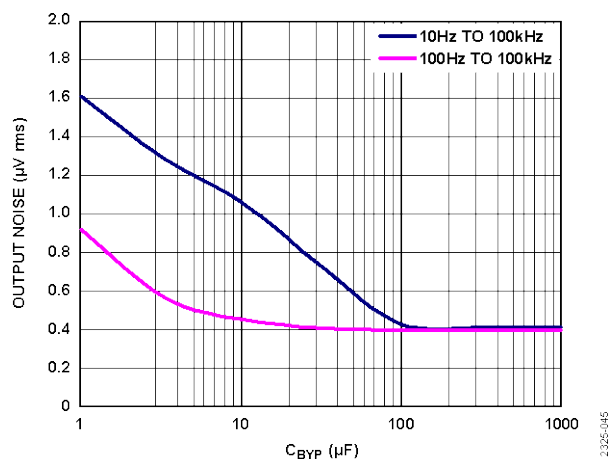
Figure 46. RMS Noise vs. C_{\text{BYP}}
