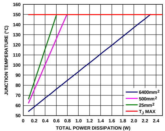
Figure 60. Junction Temperature vs. Total Power Dissipation for the 8-Lead SOIC, T_A = 50^\circ\text{C}
