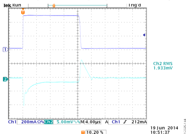
Figure 45. Output Transient Response, V_{\text{OUT}} = 3.3\text{ V} , C_{\text{OUT}} = 10\text{ }\mu\text{F} , CH1 = Load Current, CH2 = V_{\text{OUT}}
