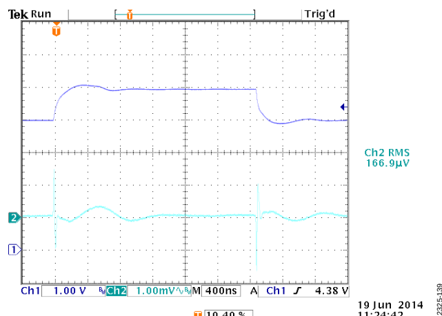
Figure 39. Line Transient Response, 1 V Input Step, I_{LOAD} = 600 \text{ mA} , V_{OUT} = 3.3 \text{ V} , V_{IN} = 3.9 \text{ V} , CH1 = V_{IN} , CH2 = V_{OUT}
