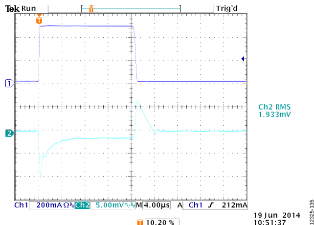
Figure 35. Load Transient Response, I_{LOAD} = 10 \text{ mA} to 510 \text{ mA} , V_{OUT} = 3.3 \text{ V} , V_{IN} = 3.8 \text{ V} , CH1 = I_{OUT} , CH2 = V_{OUT}
