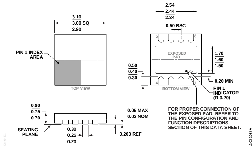
Figure 66. 8-Lead Lead Frame Chip Scale Package [LFCSP_WD] 3 mm × 3 mm Body, Very Very Thin, Dual Lead (CP-8-21) Dimensions shown in millimeters
