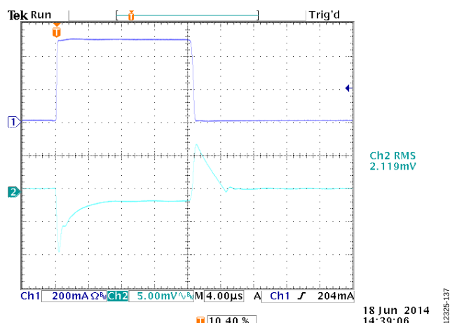
Figure 37. Load Transient Response, I_{LOAD} = 10 \text{ mA} to 510 \text{ mA} , V_{OUT} = 1.8 \text{ V} , V_{IN} = 2.3 \text{ V} , CH1 = I_{OUT} , CH2 = V_{OUT}
