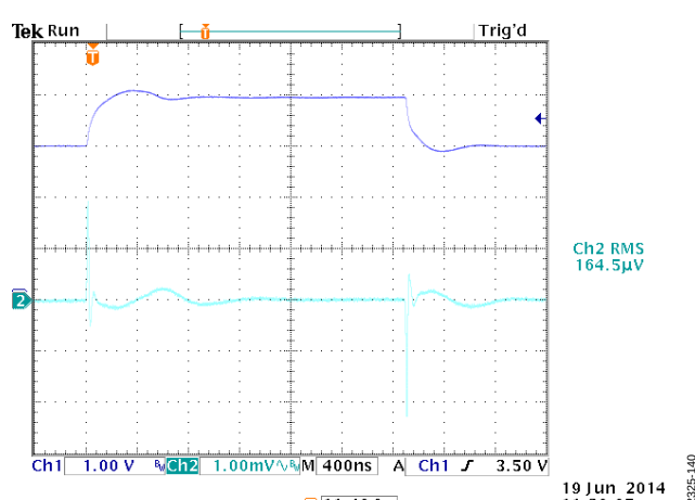
Figure 40. Line Transient Response, 1 V Input Step, I_{LOAD} = 600 \text{ mA} , V_{OUT} = 1.8 \text{ V} , V_{IN} = 2.4 \text{ V} , CH1 = V_{IN} , CH2 = V_{OUT}
