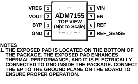
Figure 4. 8-Lead SOIC Pin Configuration
