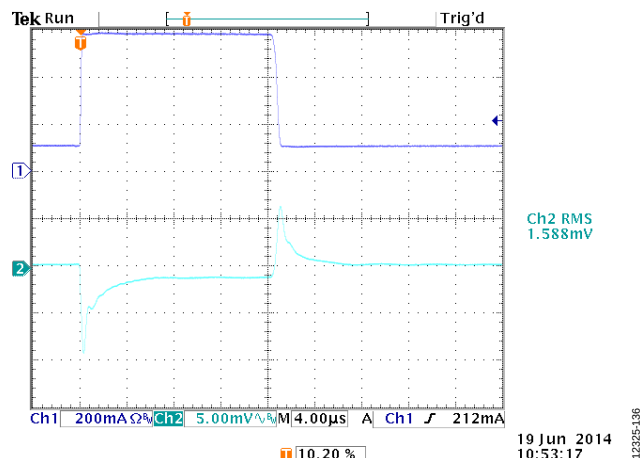
Figure 36. Load Transient Response, I_{LOAD} = 100 \text{ mA} to 600 \text{ mA} , V_{OUT} = 3.3 \text{ V} , V_{IN} = 3.8 \text{ V} , CH1 = I_{OUT} , CH2 = V_{OUT}
