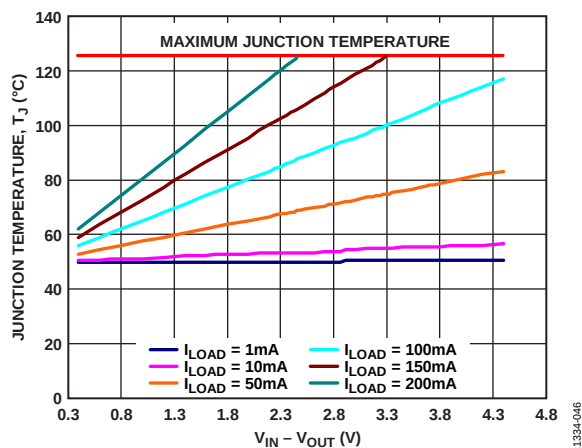
Figure 48. TSOT, 50 mm 2 of PCB Copper, T_A = 50^\circ\text{C}
