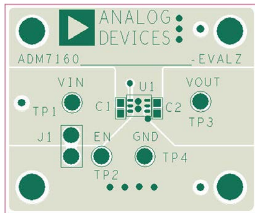
Figure 58. Example of PCB Layout, LFCSP Package
