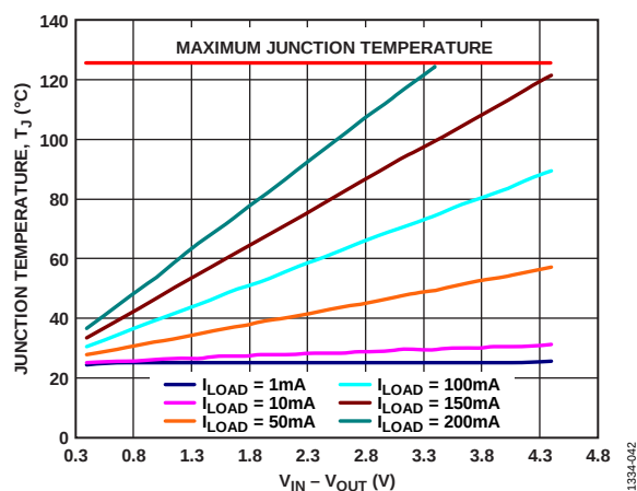
Figure 44. TSOT, 100 mm 2 of PCB Copper, T_A = 25^\circ\text{C}
