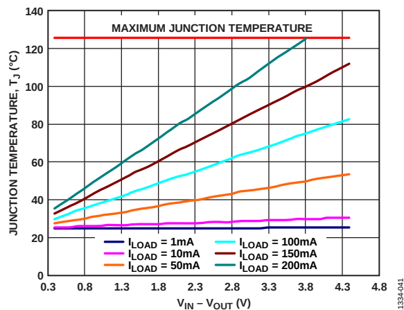
Figure 43. TSOT, 500 mm 2 of PCB Copper, T_A = 25^\circ\text{C}
