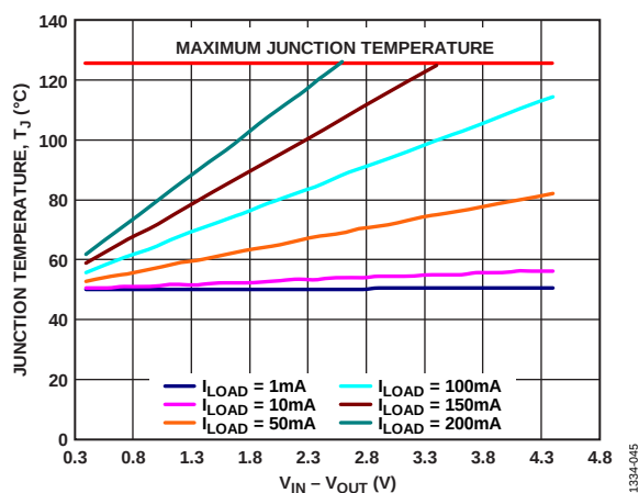
Figure 47. TSOT, 100 mm 2 of PCB Copper, T_A = 50^\circ\text{C}
