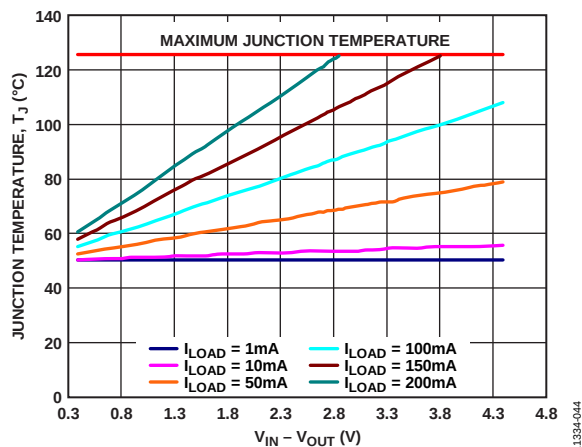
Figure 46. TSOT, 500 mm 2 of PCB Copper, T_A = 50^\circ\text{C}
