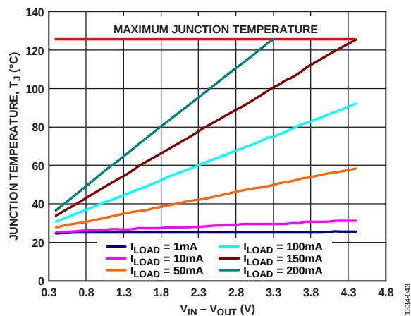
Figure 45. TSOT, 50 mm 2 of PCB Copper, T_A = 25^\circ\text{C}
