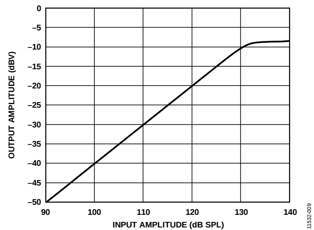
Figure 9. Linearity
