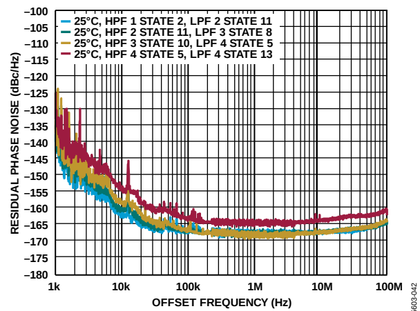
Figure 15. Residual Phase Noise vs. Offset Frequency
