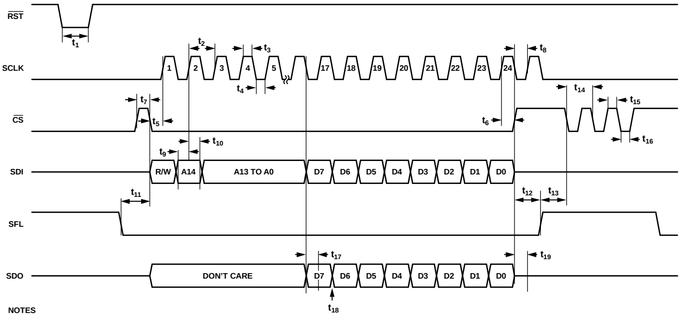
Figure 2. Timing Diagram
