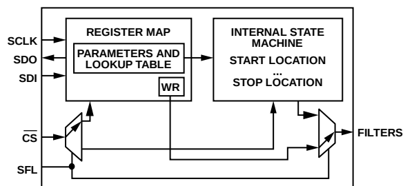
Figure 36. Simplified SPI Diagram
