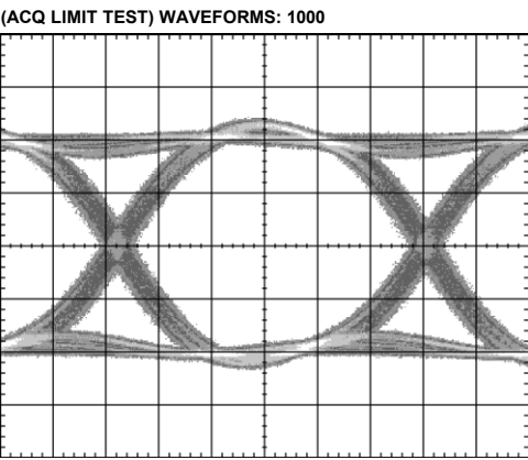
Figure 14. Electrical Eye Diagram (10.7 Gbps, PRBS31, IMOD = 80 mA)
