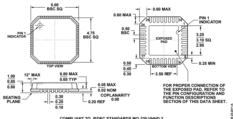
Figure 30. 32-Lead Lead Frame Chip Scale Package [LFCSP_VQ] 5 mm × 5 mm Body, Very Thin Quad (CP-32-2) Dimensions shown in millimeters
