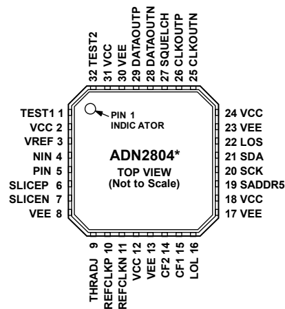
Figure 5. Pin Configuration
