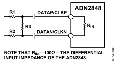
Figure 6. Attenuation Circuit
