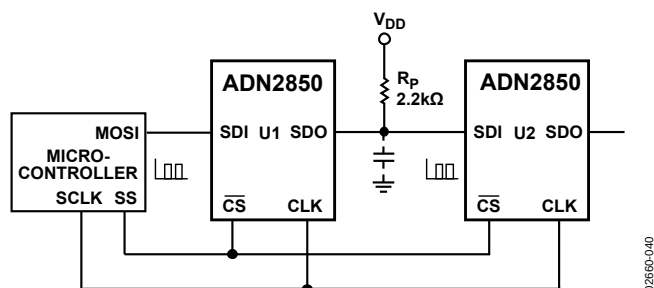
Figure 28. Daisy-Chain Configuration Using SDO
