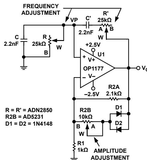
Figure 36. Programmable Oscillator with Amplitude Control
