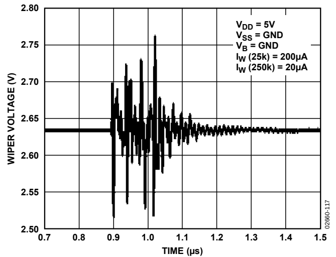
Figure 17. Digital Feedthrough
