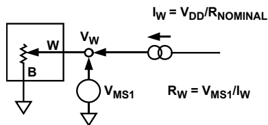
Figure 21. Wiper Resistance
