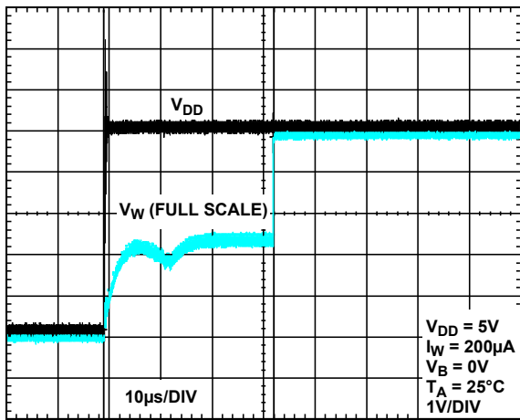
Figure 14. Power-On Reset
