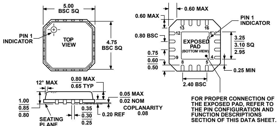
Figure 44. 16-Lead Lead Frame Chip Scale Package [LFCSP_VQ] 5 × 5 mm Body, Very Thin Quad (CP-16-6) Dimensions shown in millimeters
