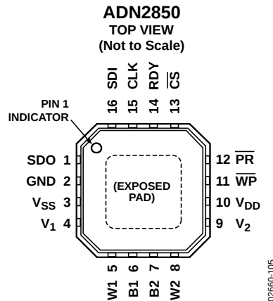
Figure 5. Pin Configuration
