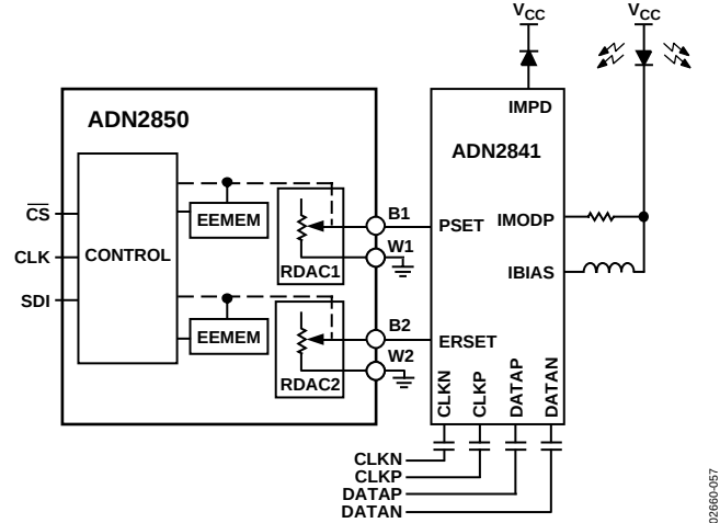
Figure 37. Optical Supervisory System
