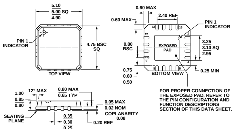
Figure 44. 16-Lead Lead Frame Chip Scale Package [LFCSP_VQ]
