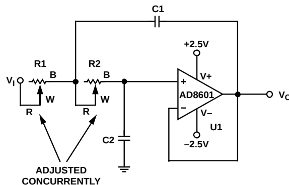
Figure 35. Sallen-Key Low-Pass Filter
