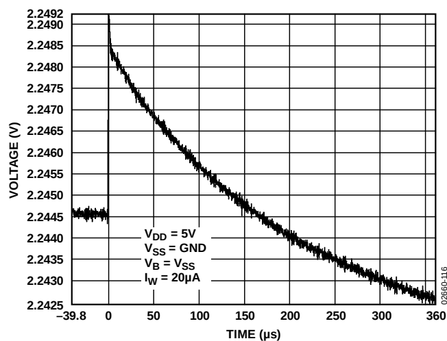
Figure 16. Midscale Glitch Energy, R_{AB} = 250\text{ k}\Omega , Code 0x200 to Code 0x1FF
