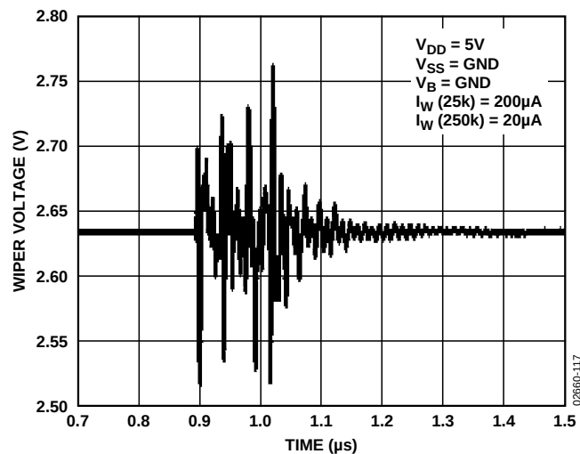
Figure 17. Digital Feedthrough
