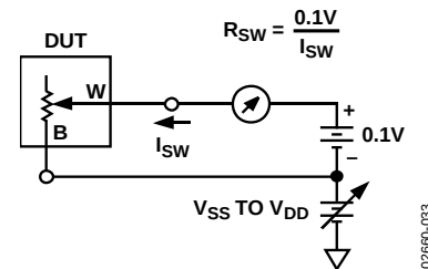
Figure 23. Incremental On Resistance
