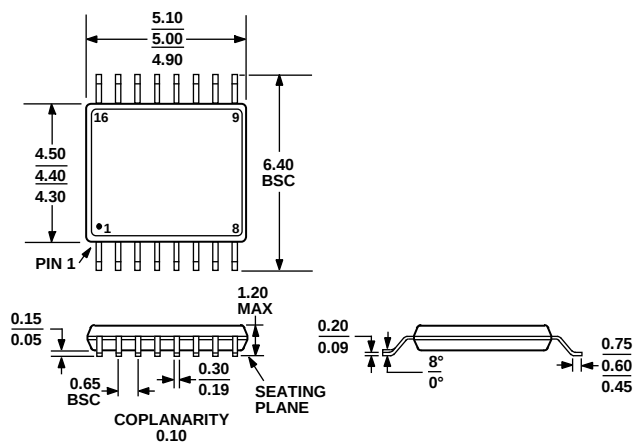
Figure 45. 16-Lead Thin Shrink Small Outline Package [TSSOP]
