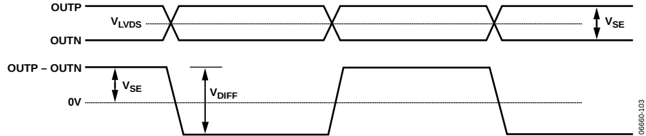
Figure 3. Single-Ended vs. Differential Output Specifications
