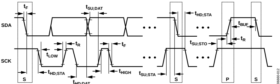
Figure 14. I 2 C Port Timing Diagram
