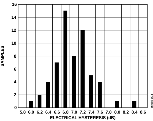
Figure 8. Sample Lot Distribution—Worst-Case Condition: Conditions = 4.25 Gbps, 100 kΩ @ -40°C, 3.6 V
