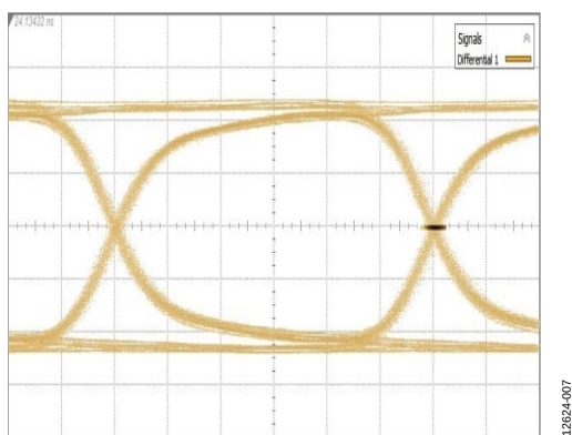
Figure 6. Output Eye Diagram at \text{CPRI} \times 16 = 9.8304\text{ Gbps} , Time = 16.95 ps/div, Amplitude = 116 mV/div
