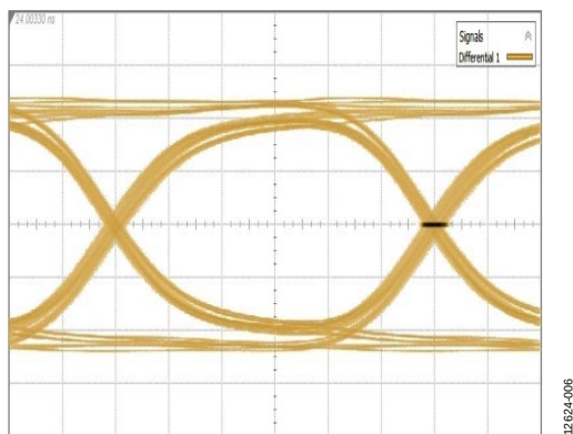
Figure 6. Output Eye Diagram at \text{CPRI} \times 16 = 9.8304\text{ Gbps} , Time = 16.95 ps/div, Amplitude = 116 mV/div
