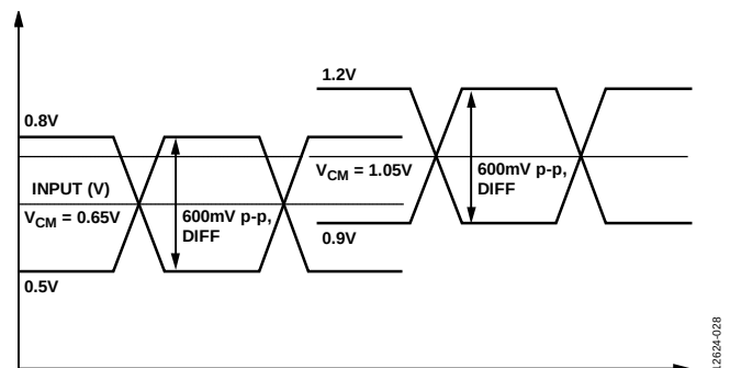
Figure 28. Minimum Allowed DC-Coupled Input Levels
