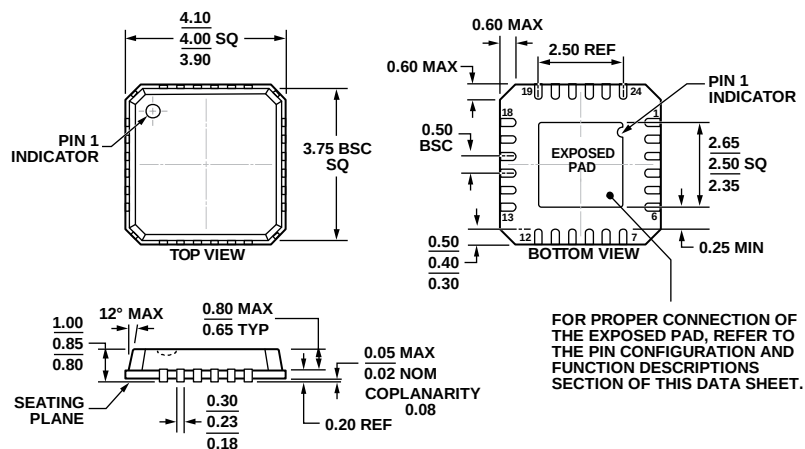
Figure 30. 24-Lead Lead Frame Chip Scale Package [LFCSP_VQ] 4 mm × 4 mm Body, Very Thin Quad (CP-24-3) Dimensions shown in millimeters
