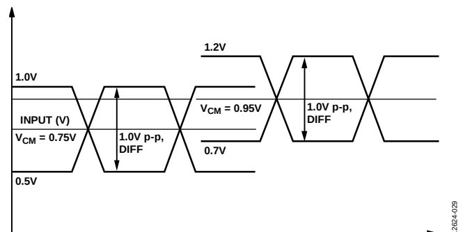
Figure 29. Maximum Allowed DC-Coupled Input Levels
