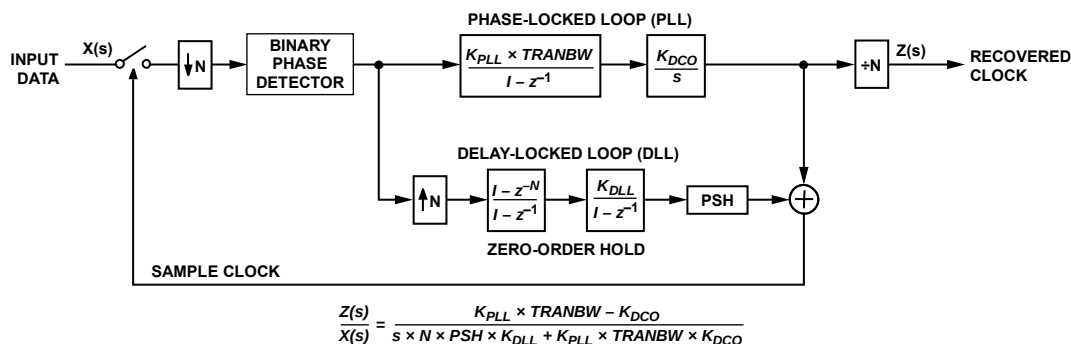
Figure 15. CDR Jitter Block Diagram
