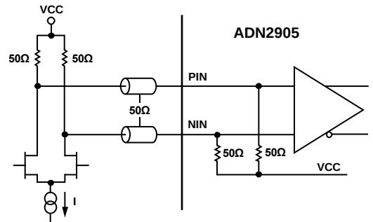
Figure 27. DC-Coupled Application, Bypass Input (Back Terminated Mode)
