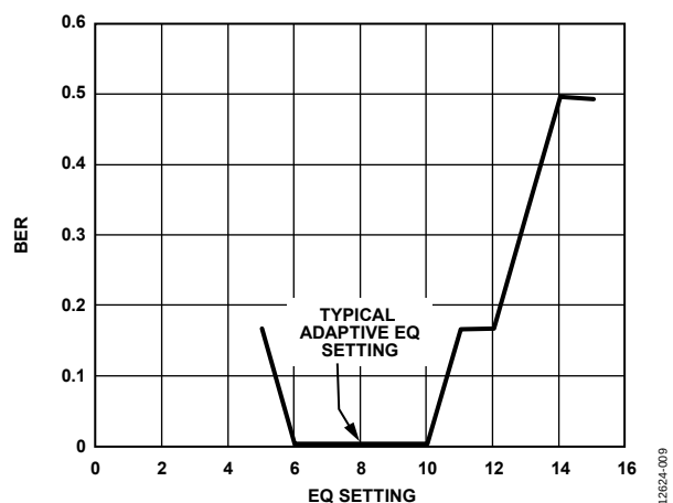
Figure 9. BER in Equalizer Mode vs. EQ Compensation at \text{CPRI} \times 16 = 9.8304\text{ Gbps} (with a Signal of 400 mV p-p Differential, on 15 inch FR4 Traces, with Variant EQ Compensation, Including Adaptive EQ)
