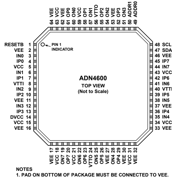
Figure 3. Pin Configuration
