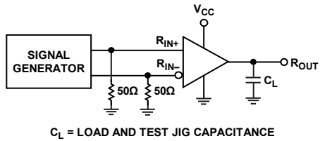
Figure 2. Test Circuit for Receiver Propagation Delay and Transition Time
