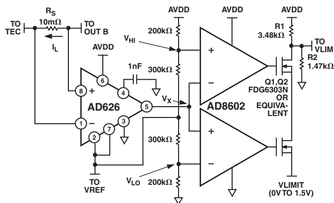
Figure 23. High Accuracy Output Current Limit
