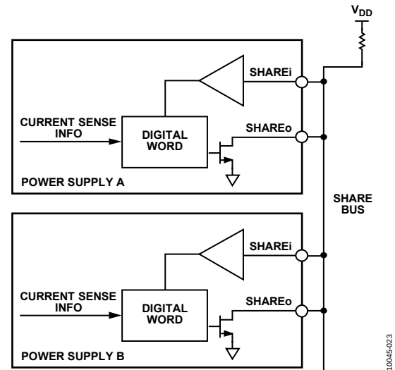
Figure 31. Digital Current Share Configuration
