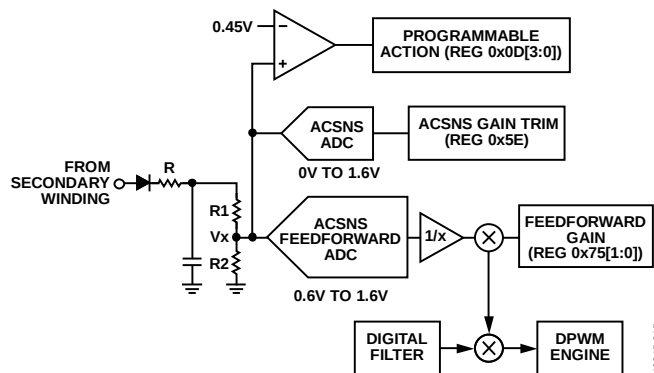
Figure 18. Feedforward Configuration
