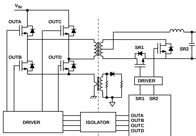
Figure 20. PWM Pin Assignment for Full-Bridge, Phase-Shifted Topology with Synchronous Rectification
