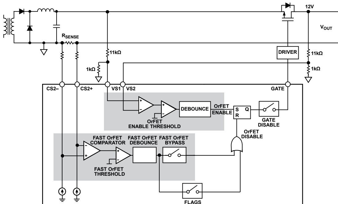
Figure 25. OrFET Control Circuit Internal Detailed Diagram
