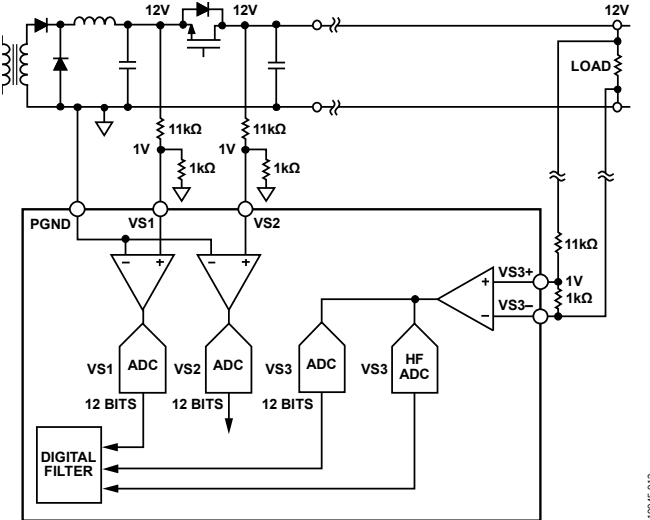
Figure 16. Voltage Sense Configuration
