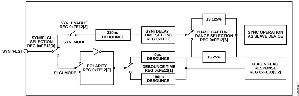
Figure 16. Synchronization Configuration
