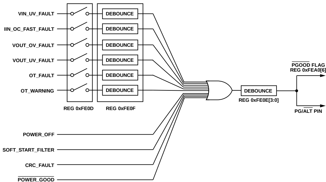
Figure 26. \overline{\text{PGOOD}} Programming
