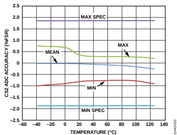
Figure 7. CS2 ADC Accuracy vs. Temperature (From 0 mV to 120 mV)
