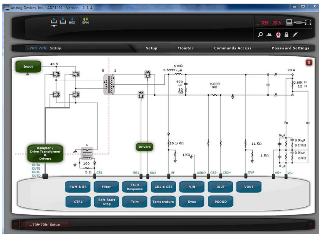
Figure 61. GUI Software
