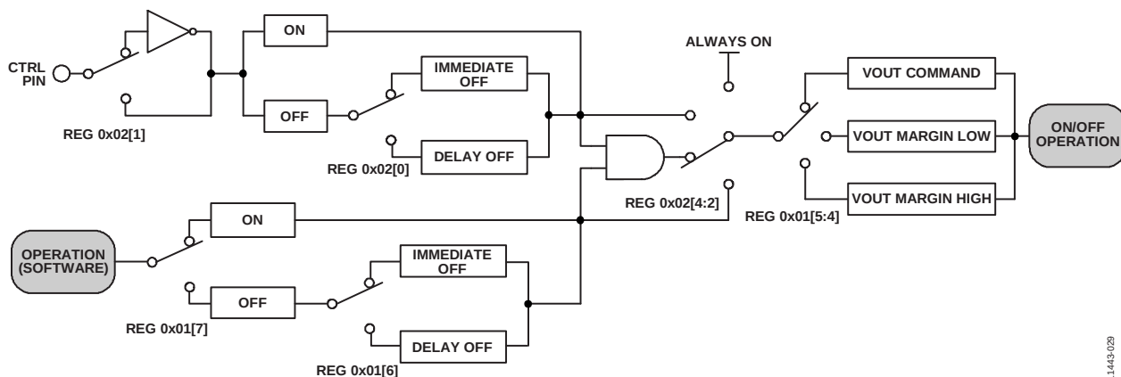
Figure 28. On/Off Control Diagram
