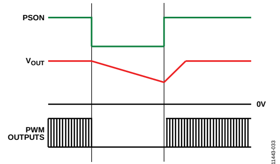
Figure 32. Pre-Bias Startup
