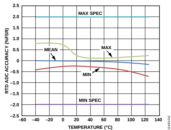
Figure 8. RTD ADC Accuracy vs. Temperature (From 10% to 90% of FSR)
