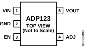
Figure 7. ADP123 TSOT Adjustable Output Pin Configuration
