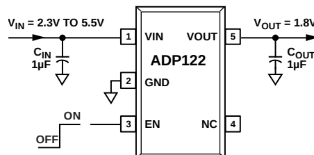
Figure 1. ADP122 with Fixed Output Voltage (TSOT Version)
