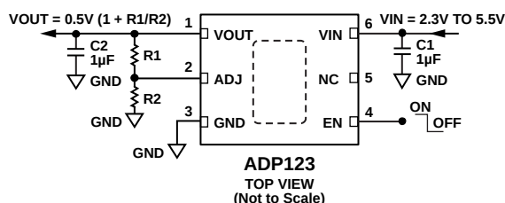
NC = NOT CONNECT. THIS PIN CAN BE LEFT FLOATING OR CONNECTED TO GROUND.
