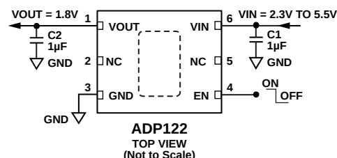
NC = NOT CONNECT. THIS PIN CAN BE LEFT FLOATING OR CONNECTED TO GROUND.
