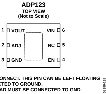
Figure 8. ADP123 LFCSP Adjustable Output Pin Configuration
