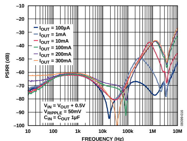
Figure 20. Power Supply Rejection Ratio vs. Frequency, V_{OUT} = 3.3\text{ V} , V_{IN} = 3.8\text{ V}
