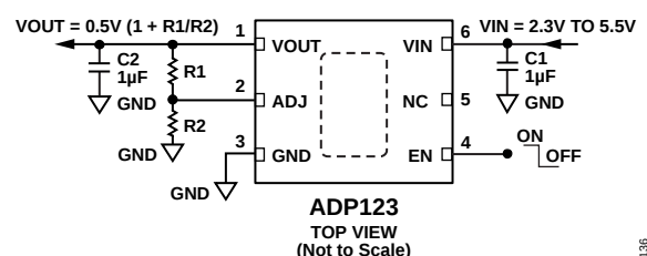
Figure 4. ADP123 with Adjustable Output Voltage (LFCSP Version)
