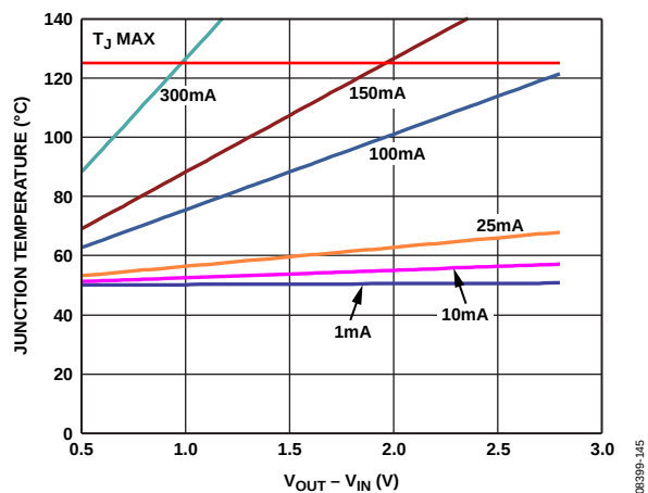
Figure 50. Junction Temperature vs. Power Dissipation, 0 mm 2 of PCB Copper, T_A = 50^\circ\text{C}
