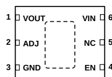
ADP123 TOP VIEW (Not to Scale)
