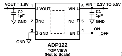
Figure 3. ADP122 with Fixed Output Voltage (LFCSP Version)
