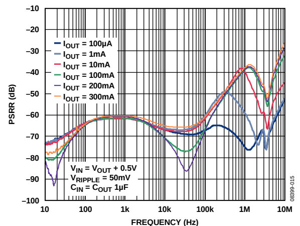
Figure 19. Power Supply Rejection Ratio vs. Frequency, V_{OUT} = 2.8\text{ V} , V_{IN} = 3.3\text{ V}
