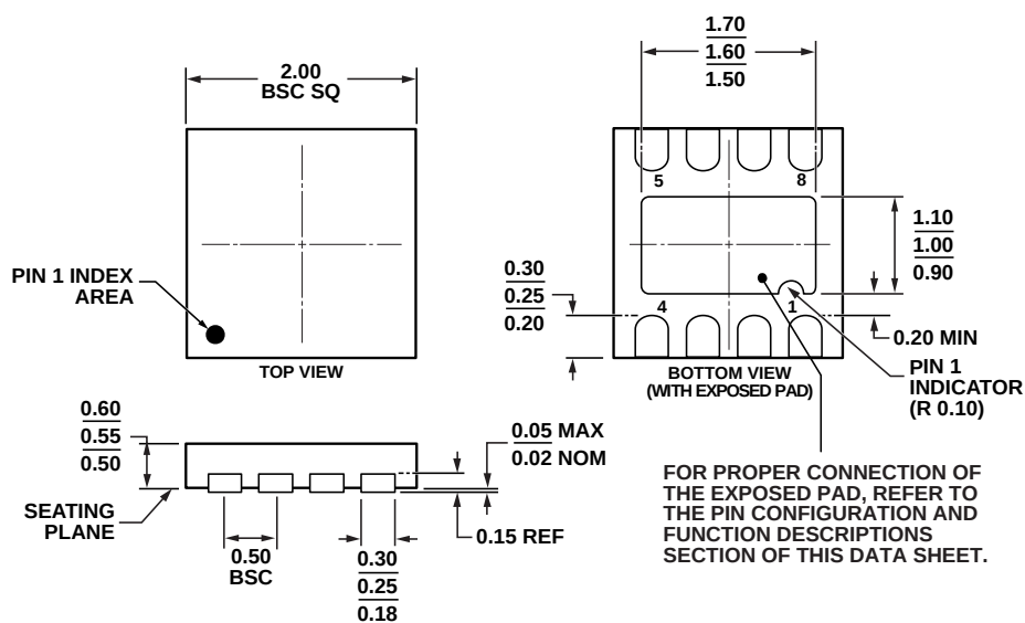
Figure 46. 8-Lead Lead Frame Chip Scale Package [LFCSP_UD] 2 mm x 2 mm Body, Ultra Thin, Dual Lead (CP-8-8)
