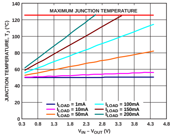
Figure 49. TSOT 100 mm² of PCB Copper, T_A = 50^\circ\text{C}
