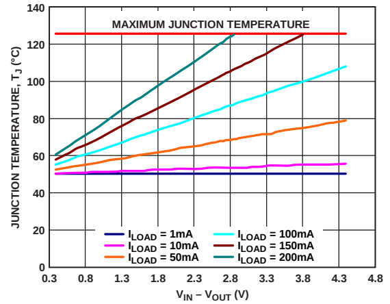
Figure 48. TSOT 500 mm² of PCB Copper, T_A = 50^\circ\text{C}
