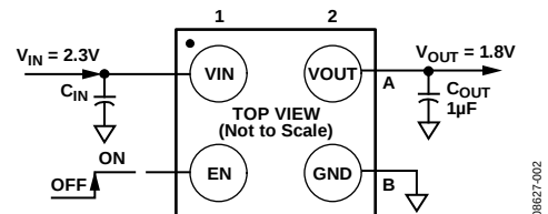
Figure 2. WLCSP ADP151 with Fixed Output Voltage, 1.8 V
