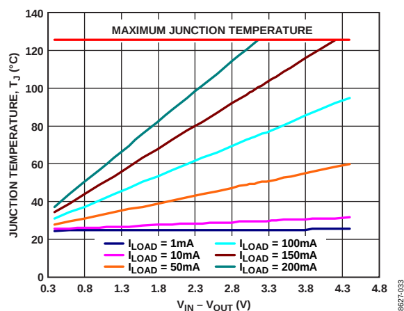
Figure 41. WLCSP 50 \text{mm}^2 of PCB Copper, T_A = 25^{\circ}\text{C}
