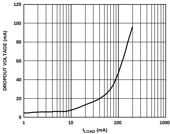
Figure 14. Dropout Voltage vs. Load Current
