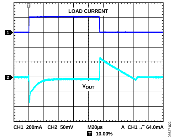
Figure 24. Load Transient Response, C_{IN} = 1\mu F , C_{OUT} = 1\mu F , I_{LOAD} = 1mA to 200mA
