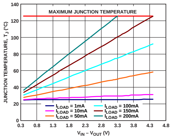
Figure 47. TSOT 50 mm² of PCB Copper, T_A = 25^\circ\text{C}
