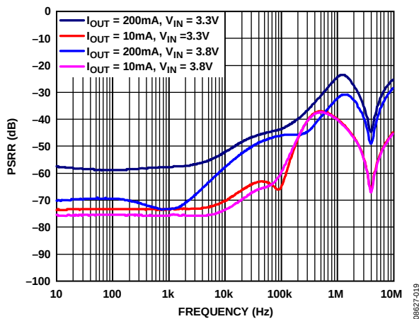
Figure 21. Power Supply Rejection Ratio vs. Frequency at Various Voltages and Load Currents, V_{OUT} = 2.8V
