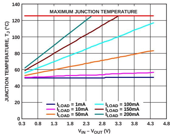
Figure 50. TSOT 50 mm² of PCB Copper, T_A = 50^\circ\text{C}
