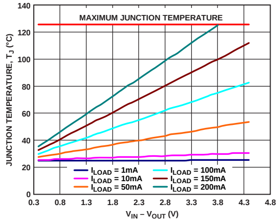
Figure 45. TSOT 500 mm² of PCB Copper, T_A = 25^\circ\text{C}
