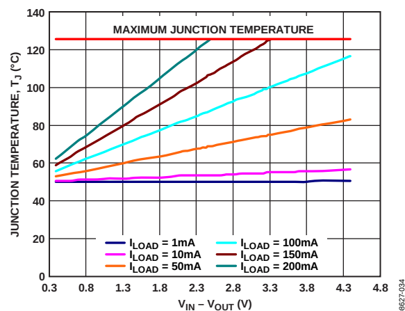
Figure 42. WLCSP 500 \text{mm}^2 of PCB Copper, T_A = 50^{\circ}\text{C}
