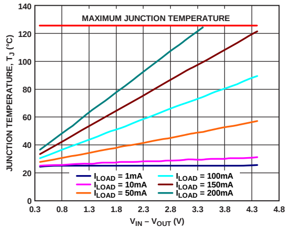
Figure 46. TSOT 100 mm² of PCB Copper, T_A = 25^\circ\text{C}
