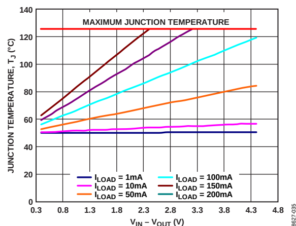
Figure 43. WLCSP 100 \text{mm}^2 of PCB Copper, T_A = 50^{\circ}\text{C}
