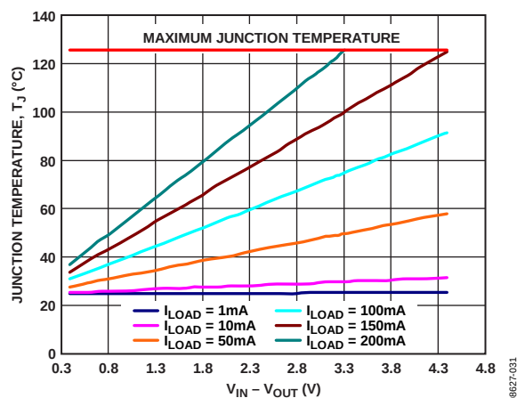
Figure 39. WLCSP 500 \text{mm}^2 of PCB Copper, T_A = 25^{\circ}\text{C}
