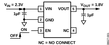
Figure 1. TSOT ADP151 with Fixed Output Voltage, 1.8 V
