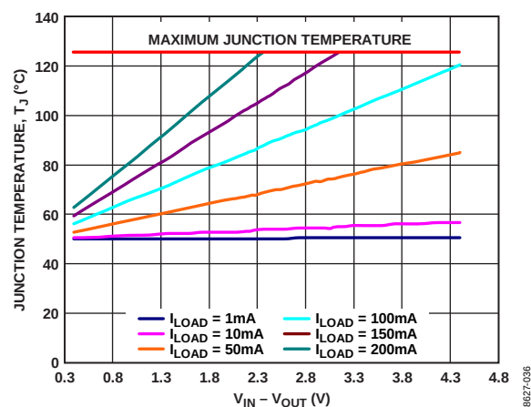
Figure 44. WLCSP 50 \text{mm}^2 of PCB Copper, T_A = 50^{\circ}\text{C}
