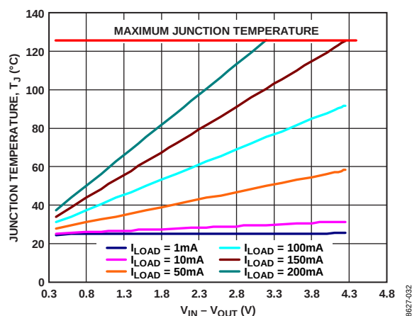
Figure 40. WLCSP 100 \text{mm}^2 of PCB Copper, T_A = 25^{\circ}\text{C}
