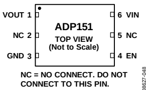
Figure 6. 6-Lead LFCSP Pin Configuration
